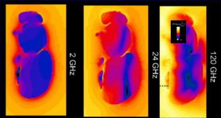
Figure 4. Normalized Electric field strength (dB) in a mid-transverse cross section of the Western Honey Bee as a function of frequency for a single plane wave incident
