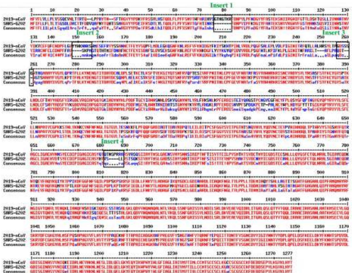
Multiple sequence alignment between spike proteins of 2019-nCoV and SARS.
