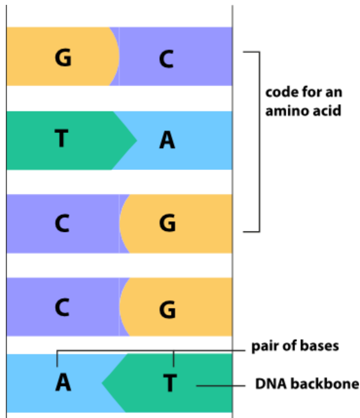
Figure 1. Paired bases within a part of the double helix
