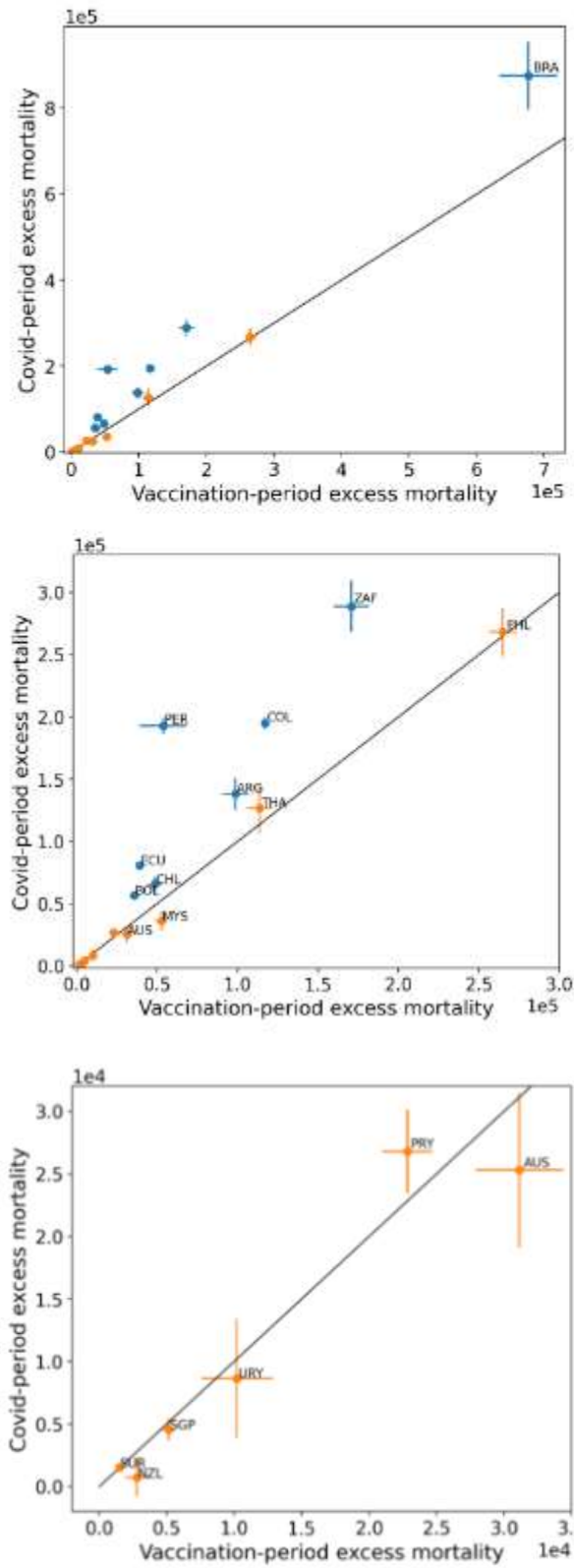
Figure 3: (three panels) Covid-period excess ACM versus vaccination-period excess ACM (top), first expanded view (middle), second expanded view (bottom), with 1:1 line as a reference.
